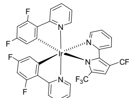
Bis(4',6'-difluorophenylpyridinato)(3,5-bis(trifluoromethyl)-2(2'-pyridyl)pyrrolate)iridium(III)
