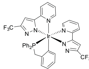
Bis(3-trifluoromethyl-5-(2-pyridyl)pyrazolate)(benzylidiphenylphosphinate)iridium(III)
