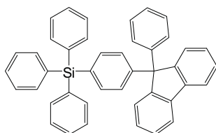
Triphenyl(4-(9-phenyl-9H-fluoren-9-yl)phenyl)silane
