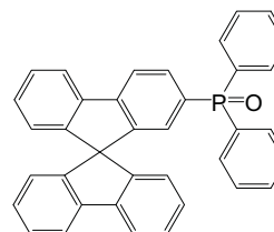
9,9-spirobifluoren-2-yl-diphenyl-phosphine oxide
