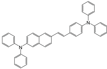
(E)-6-(4-(diphenylamino)styryl)-N,N-diphenyl-naphthalen-2-amine
