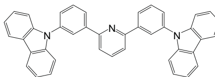
2,6-bis(3-(9H-carbazol-9-yl)phenyl)pyridine
